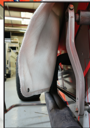
HIGH-TEMP FIBERGLASS INNER LAYER CAN REST DIRECTLY ON HEADERS WITHOUT MELTING
