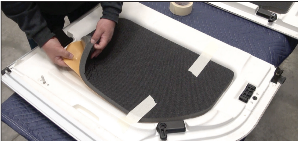
FIG. 6 Peel back a small section of release liner and adhere to freedom top section.
